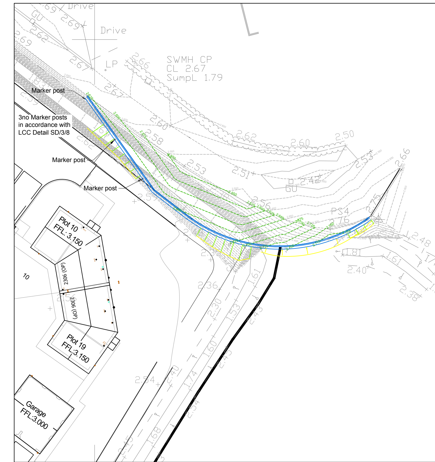
EASTERN END OF SMALL DROVE Scale 1:250
