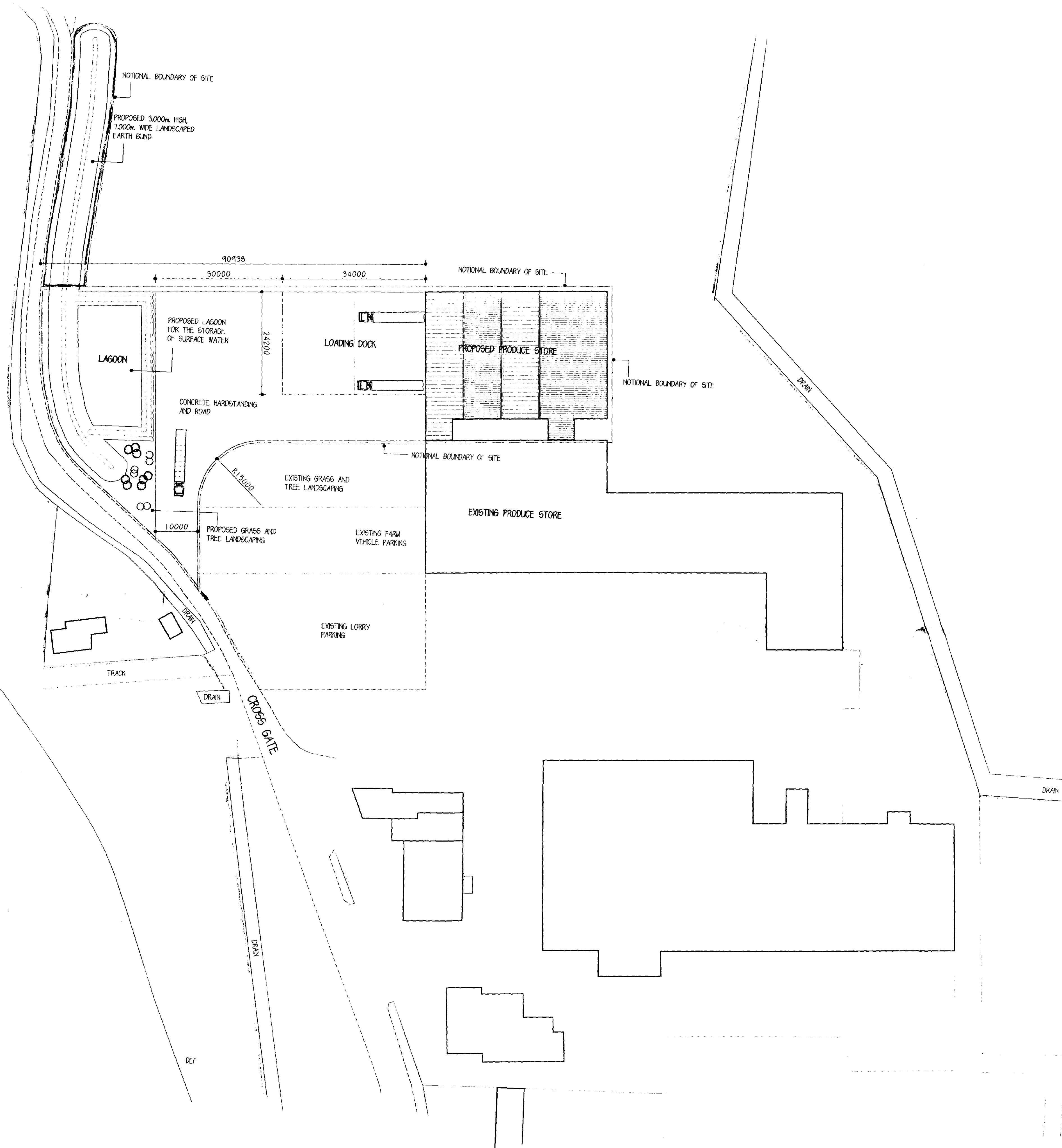
BLOCK PLAN 1:500
