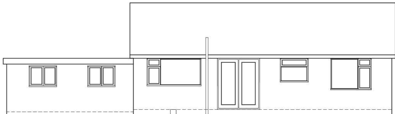
Existing Rear Elevation (East)
