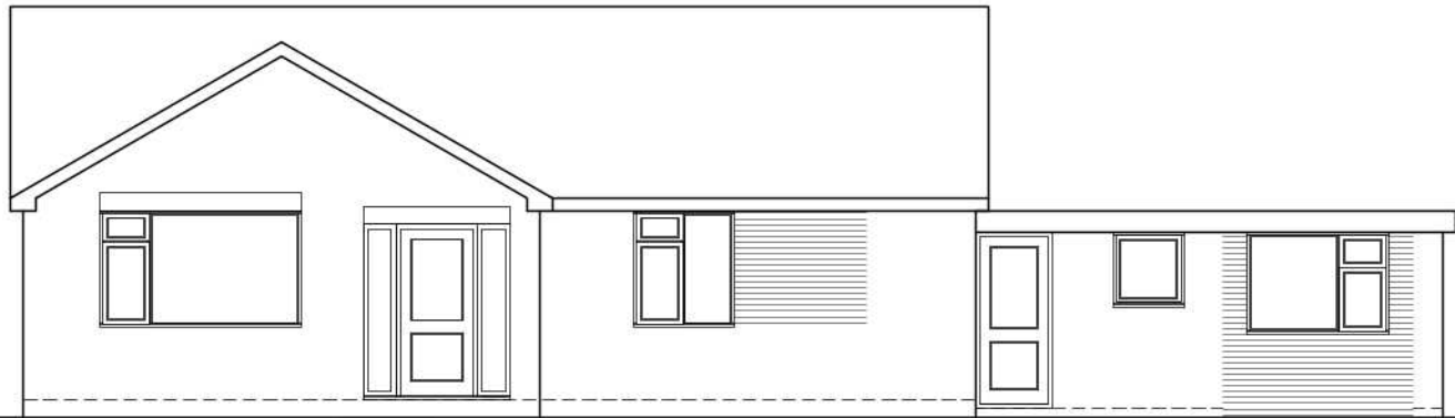
Proposed Front Elevation From Broadgate (West)
