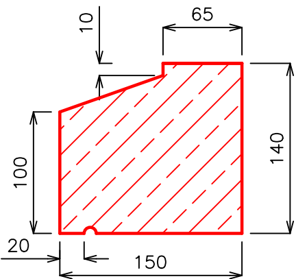
CILL PROFILE
