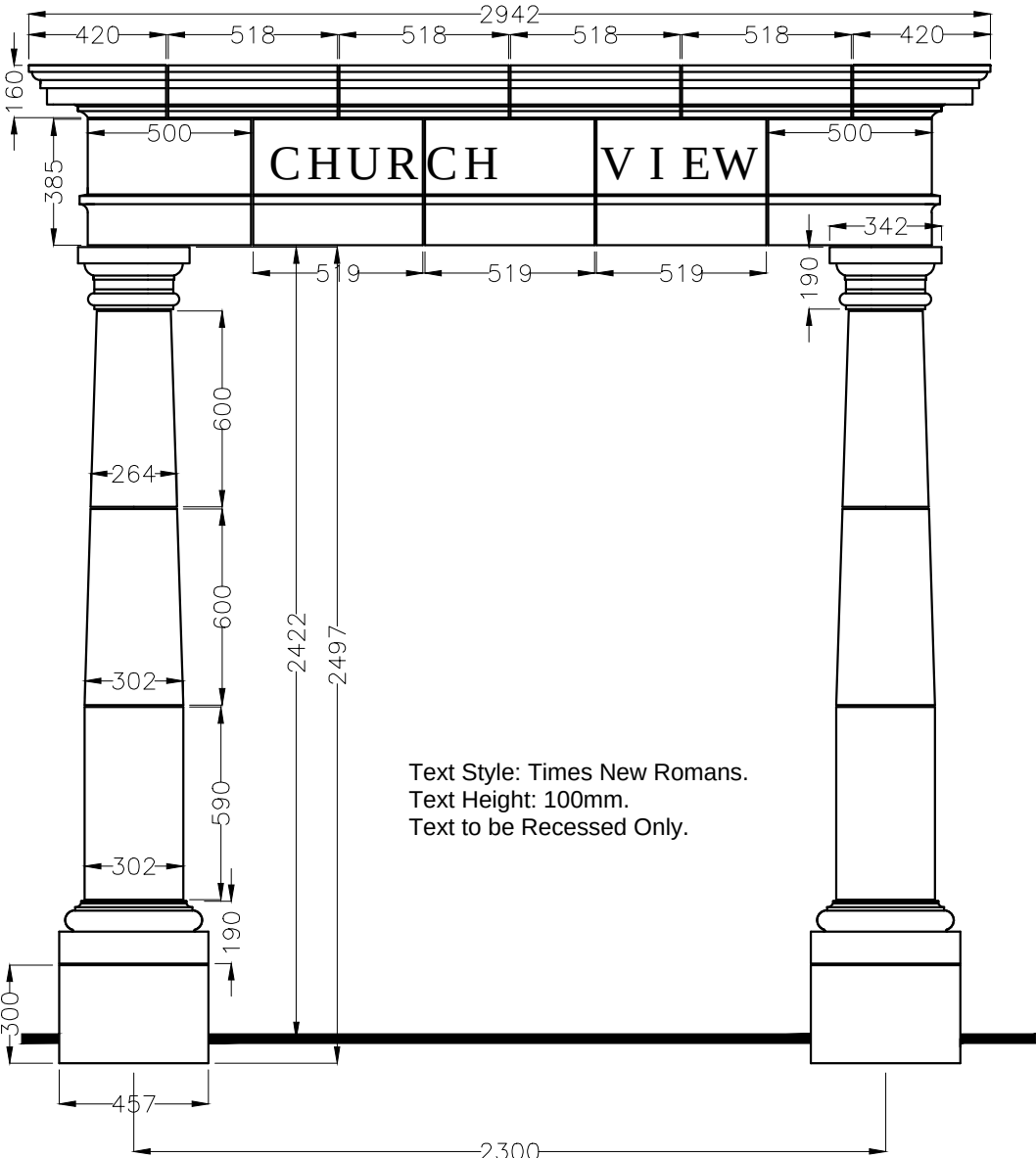
Portico - Front Elevation.
