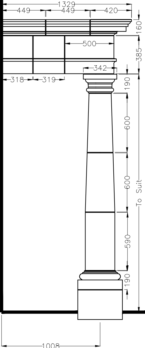
Portico - End Elevation.
