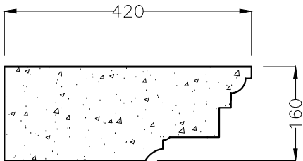
Cornice Profile.
