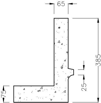
Architrave Profile.
