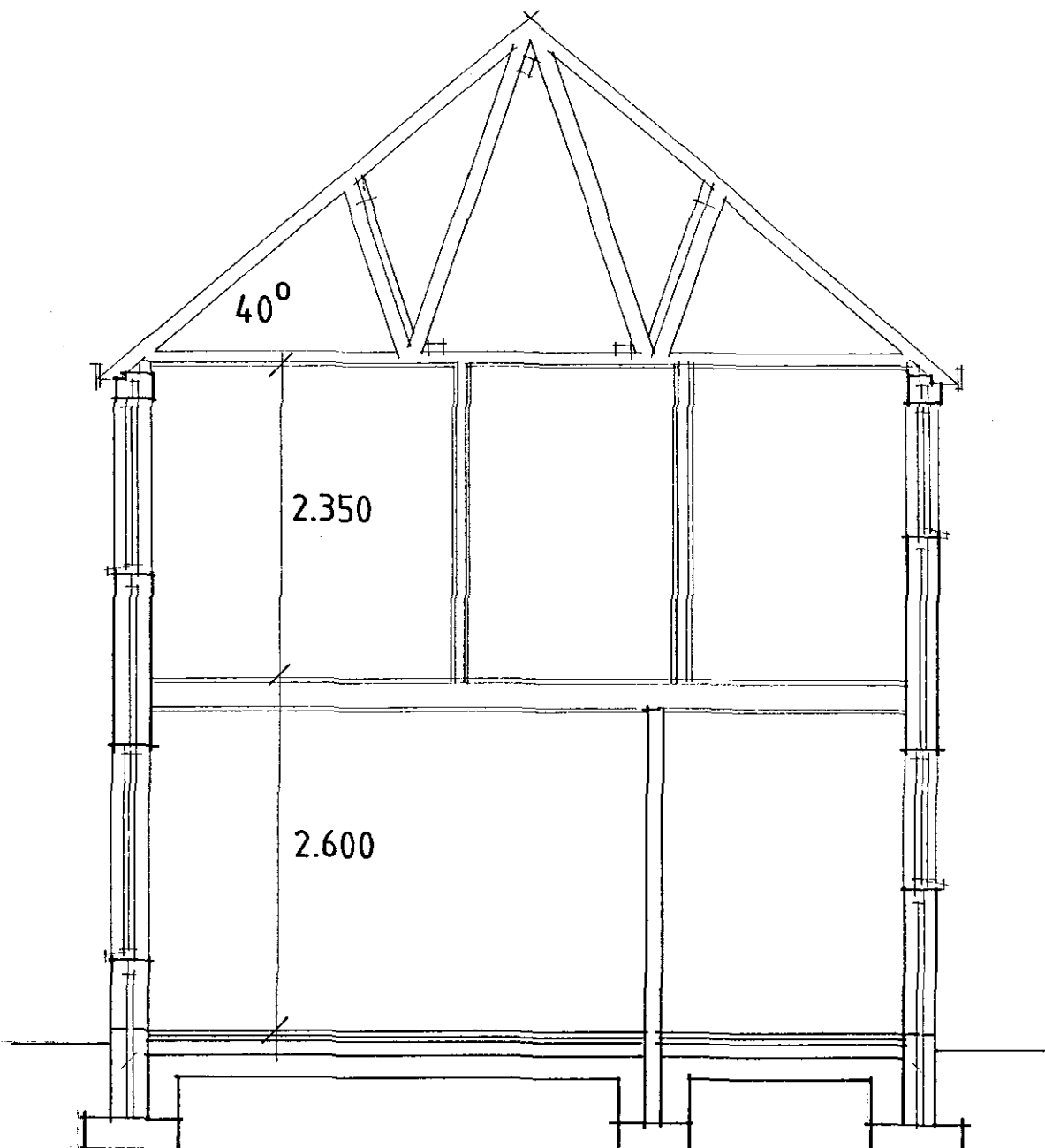
SECTION
