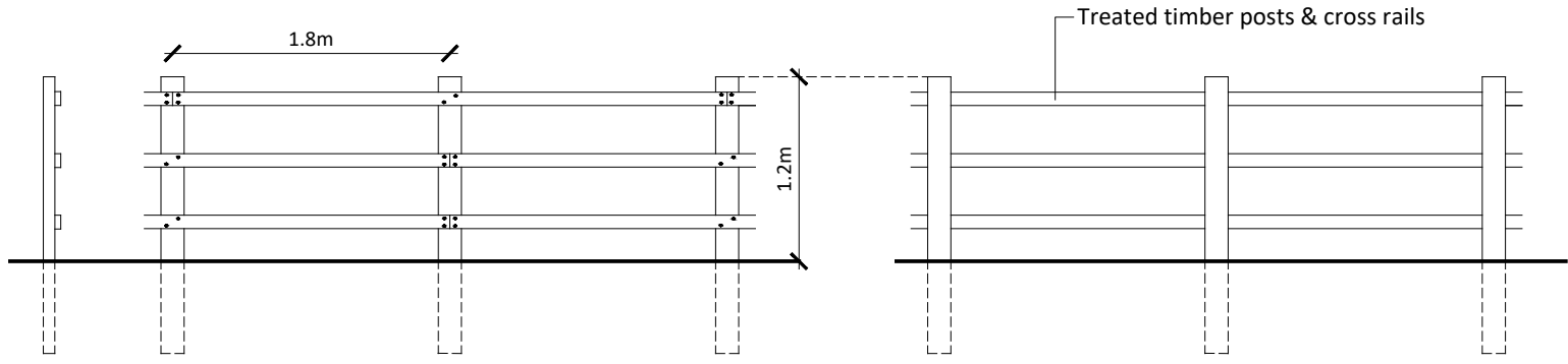
Side & front elevation
