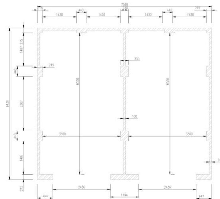
FLOOR PLANS
