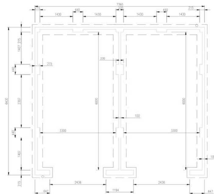
FOUNDATIONS
