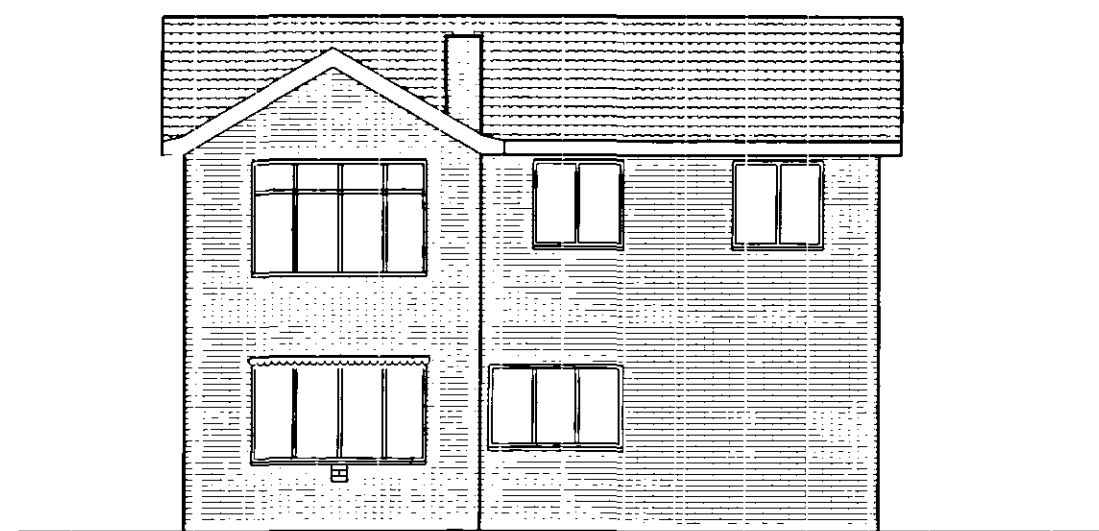
Proposed Western Elevation
