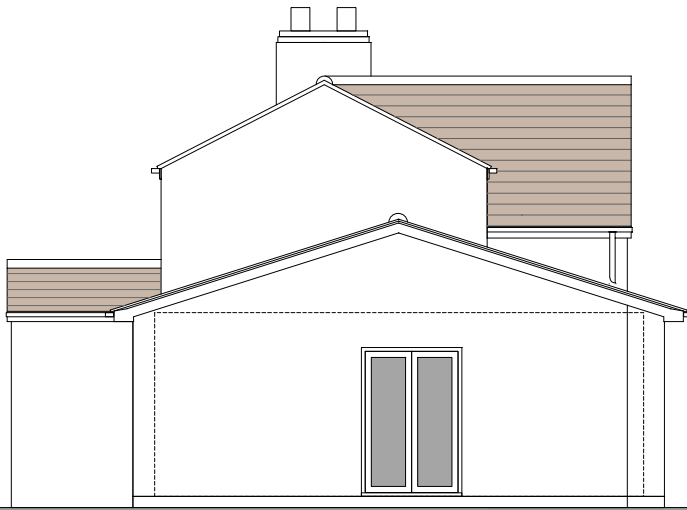
SIDE ELEVATION 2
