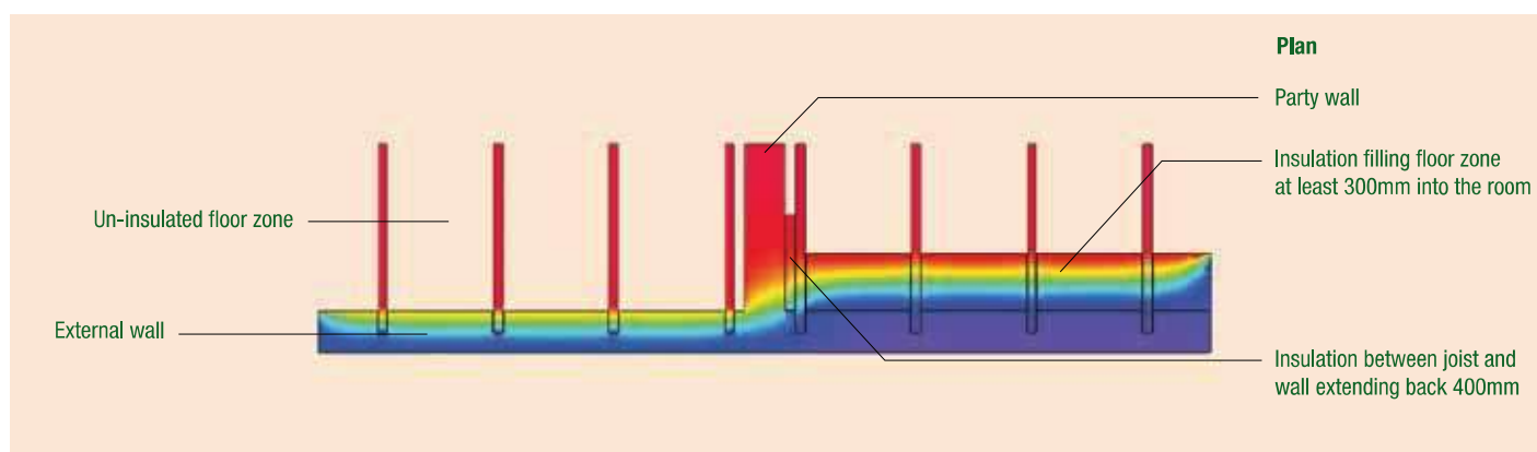
Figure 6 – Thermal contours with and without floor zone insulated (Images generated using HEAT 3 software)
