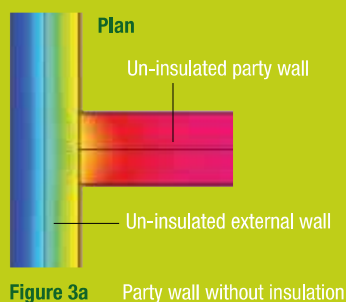
Figure 3 –Thermal contours at the junction of a 225mm solid external wall and a party wall (Images generated using HEAT 3 software)
