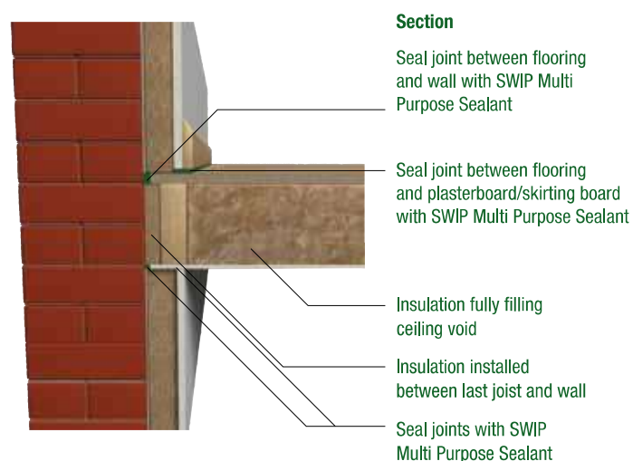
Figure 8 – Detail at intermediate timber floor
