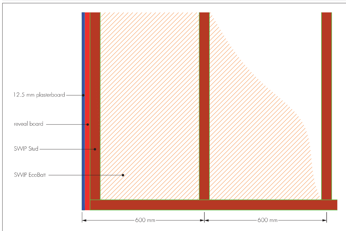
Figure 6 SWIP Stud detailing at opening
