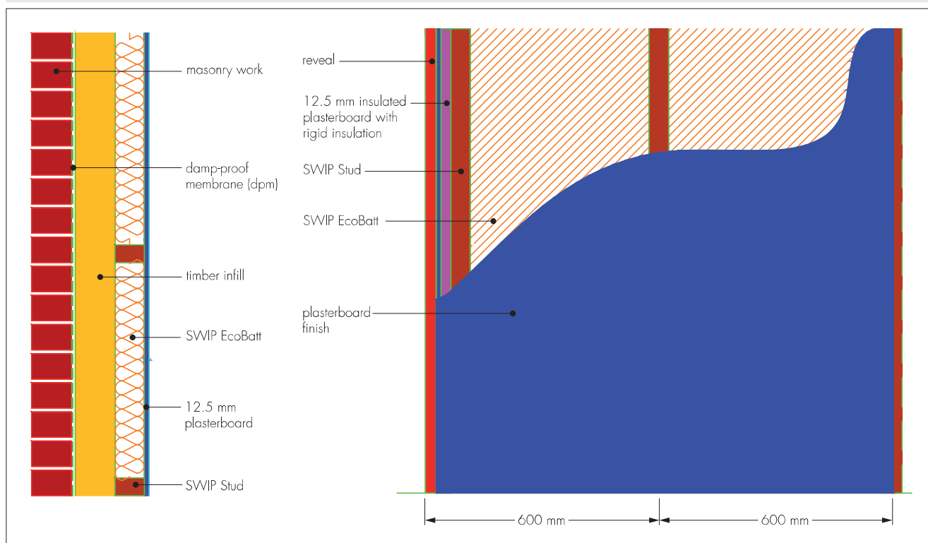
Figure 8 Stepped/checked reveal detailing
