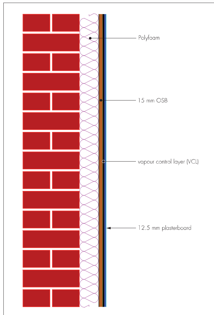
Figure 1 System side view
