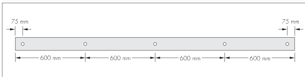
Figure 2 Fixing centres
