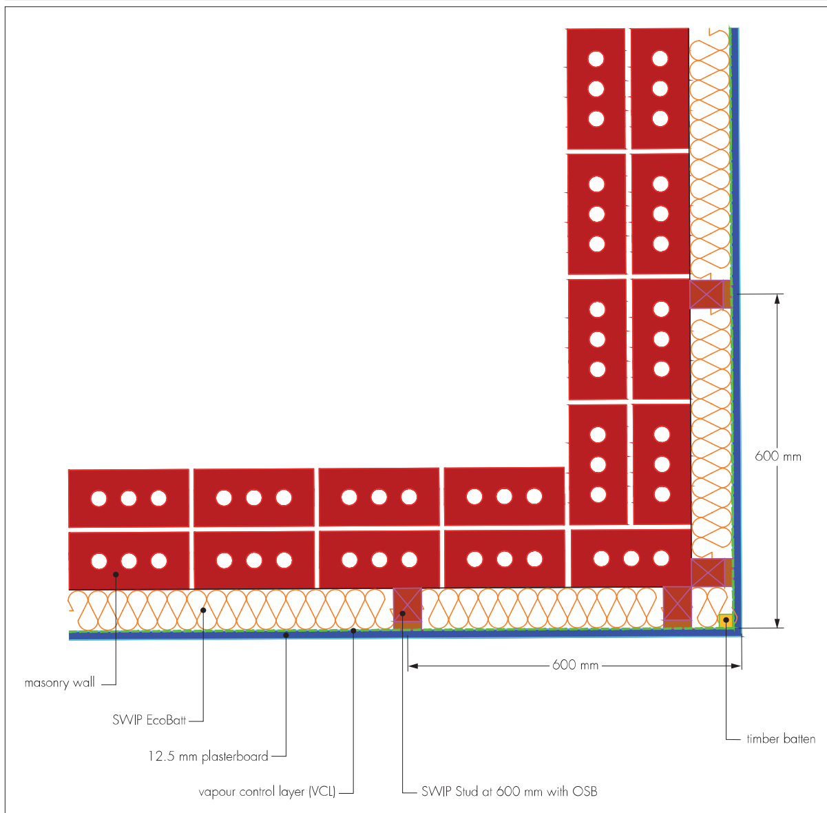
Figure 10 External corner detailing
