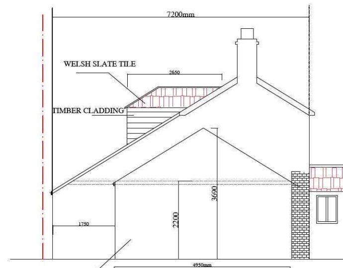
PROPOSED LEFT SIDE ELEVATION (SOUTH ELEVATION) SCALE: 1/100
