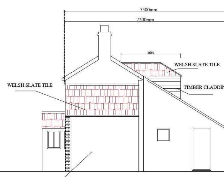
PROPOSED RIGHT SIDE ELEVATION (NORTH ELEVATION) SCALE: 1/100
