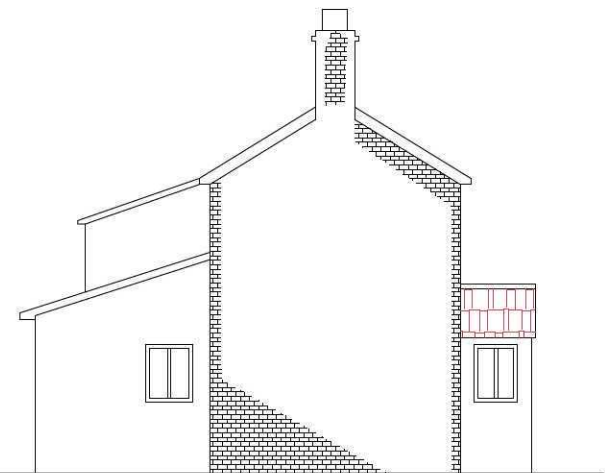
EXISTING RIGHT SIDE ELEVATION SCALE: 1/100
