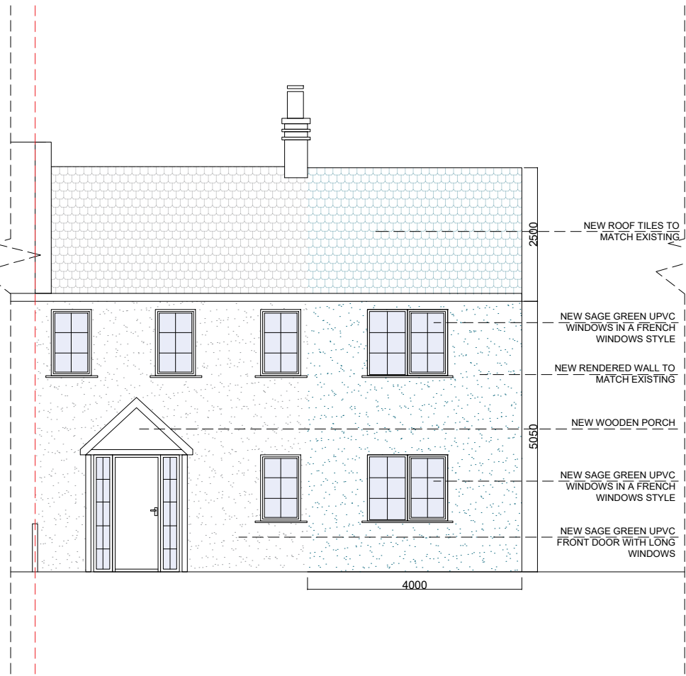
Proposed West Elevation
