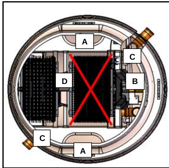
Fig. 6 - Desludge Positions
