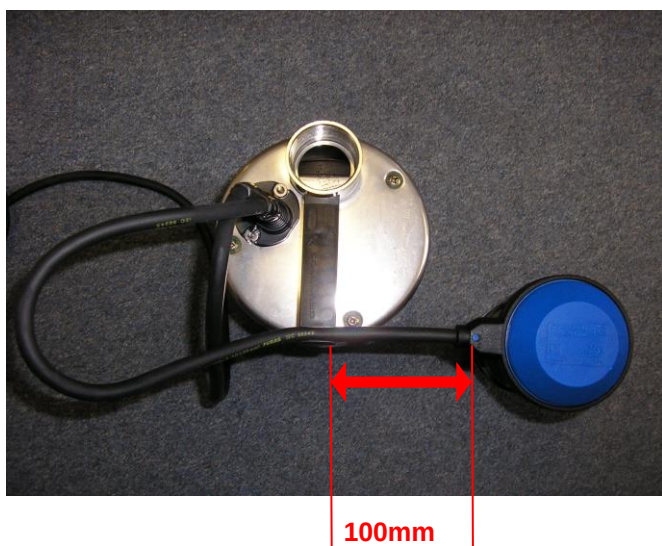
Fig. 4 - Float Setting
