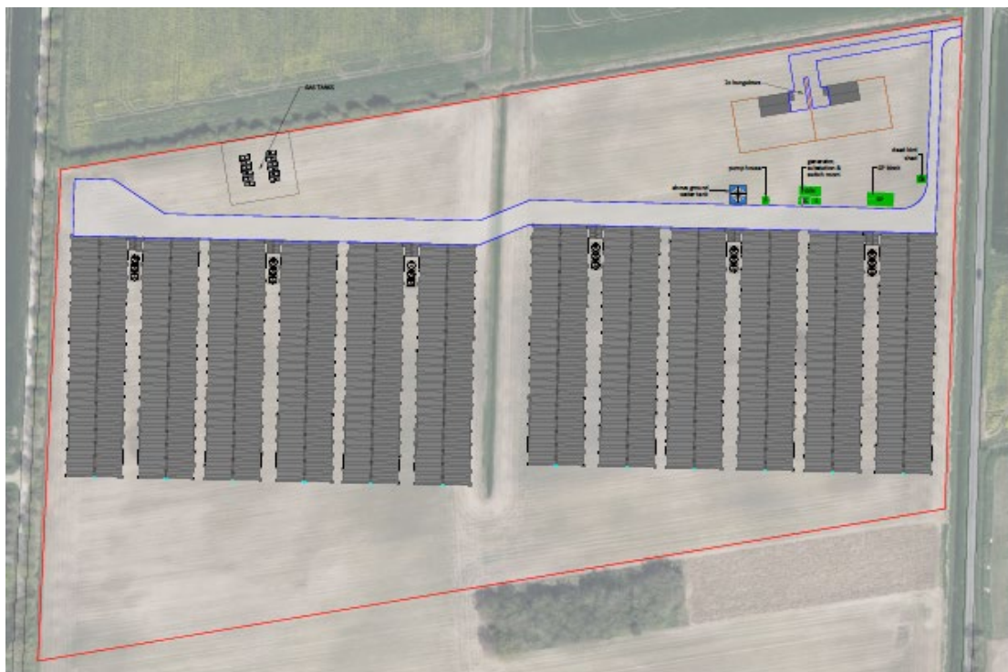
Source: Clarke Group Proposed Drawing
