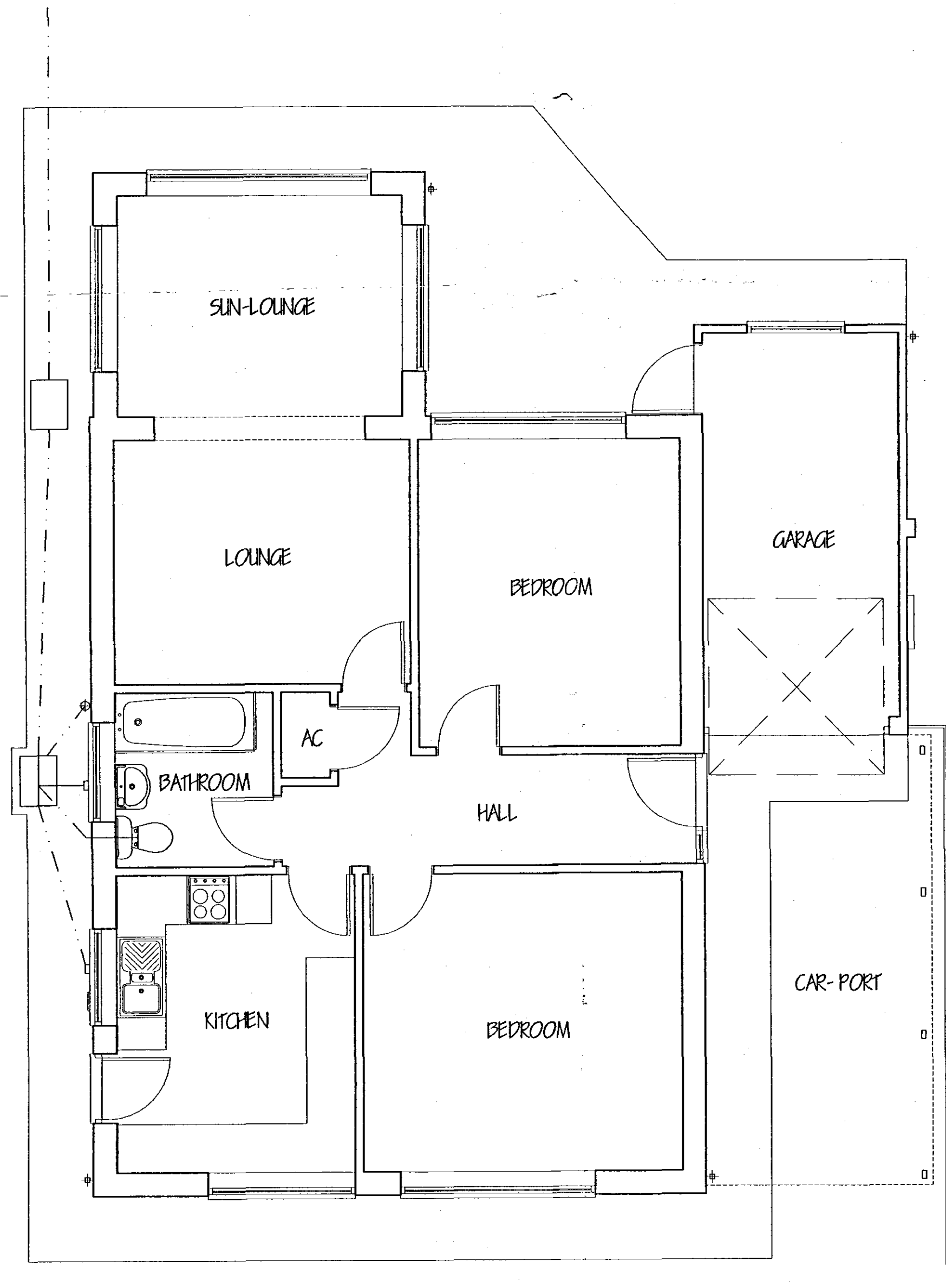
FLOOR PLAN - EXISTING.
