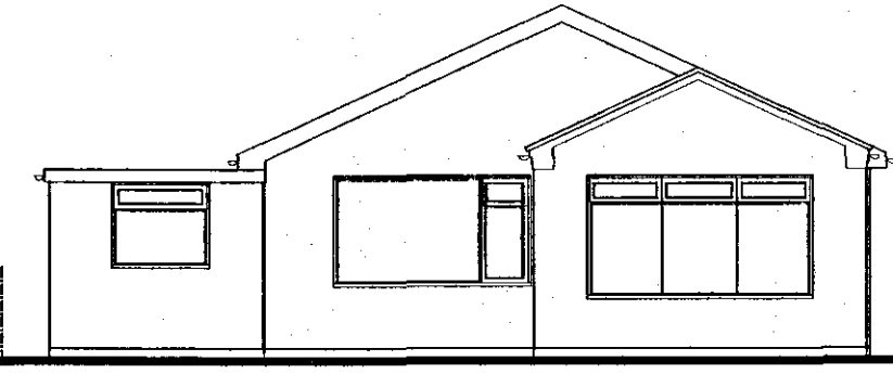
REAR ELEVATION - EXISTING.
