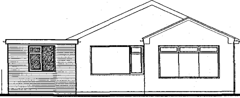
REAR ELEVATION - PROPOSED.
