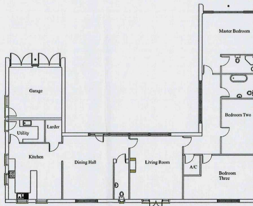
PROPOSED FLOOR LAYOUT
