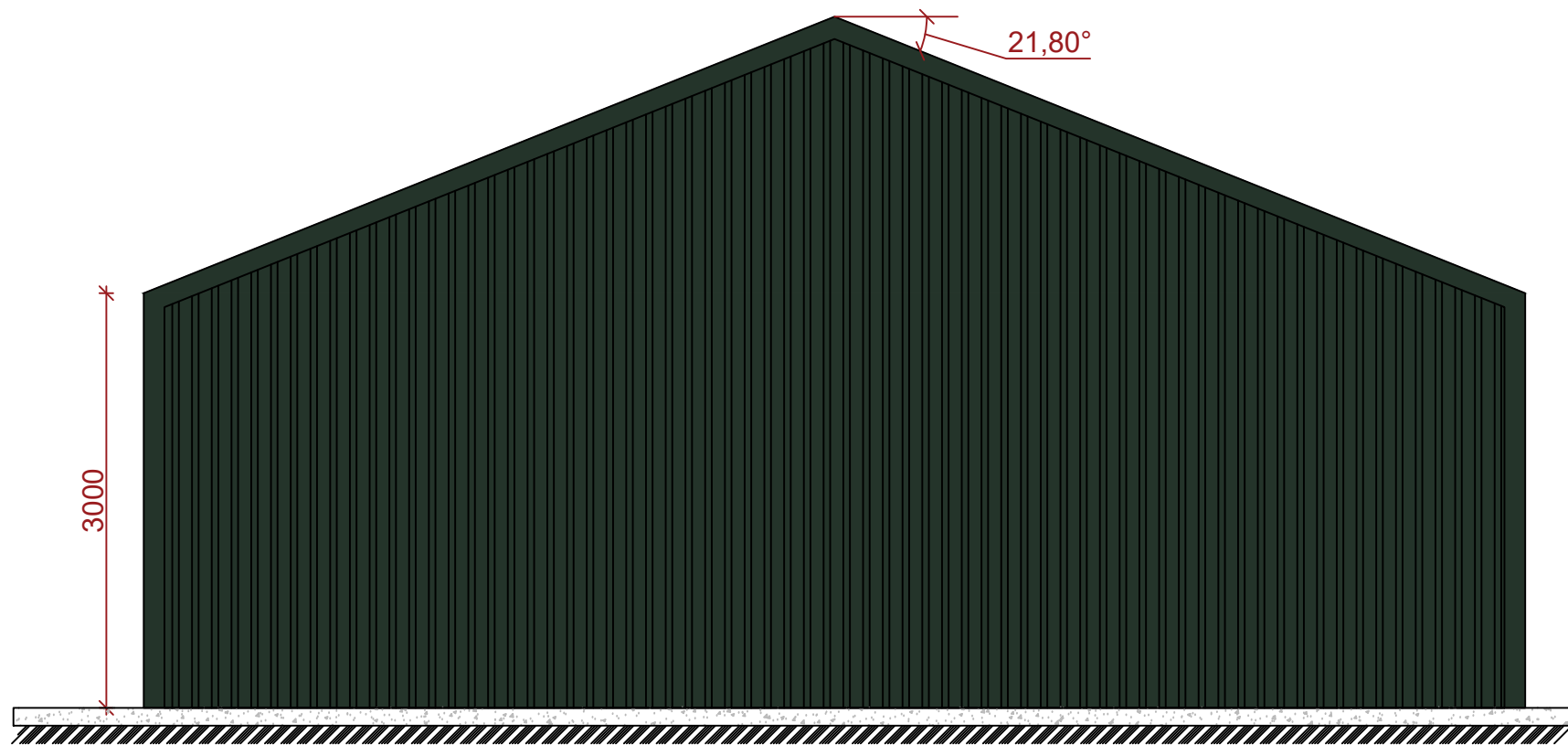
West Elevation (Rear)
