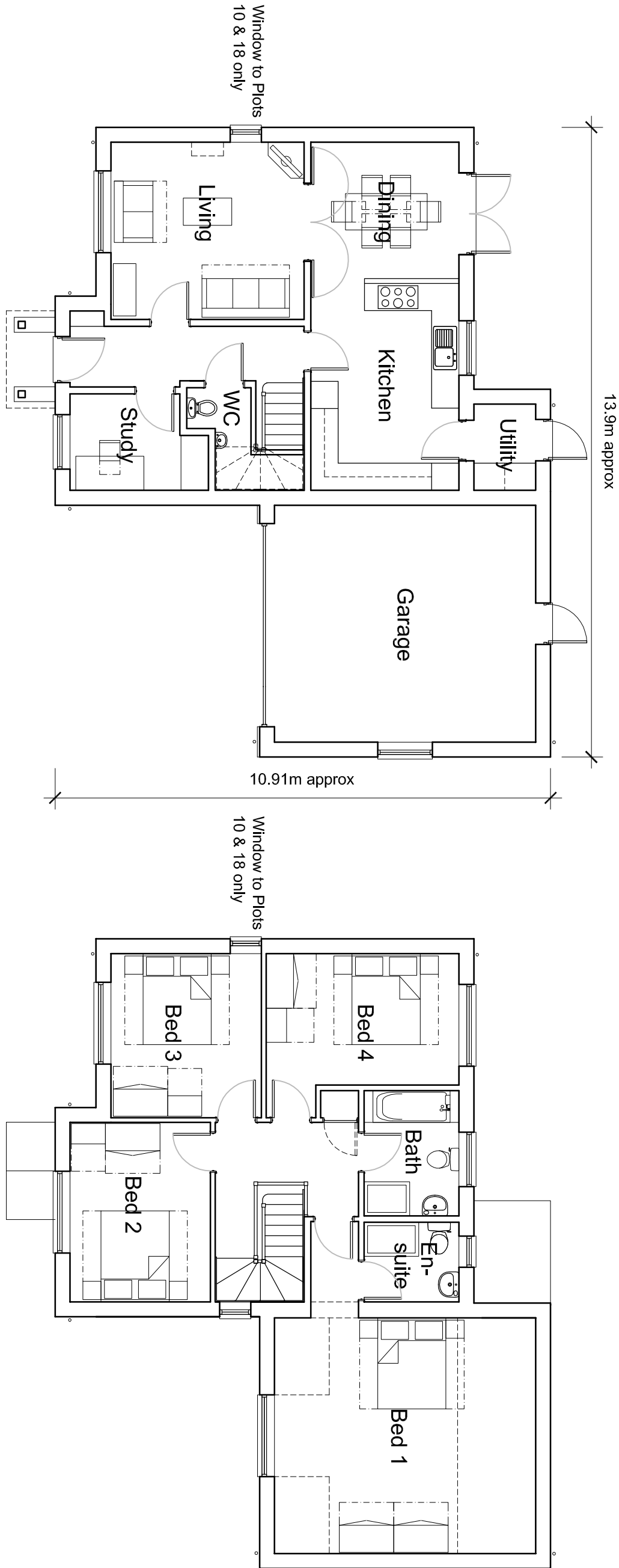
Ground Floor Plan (1:100)
