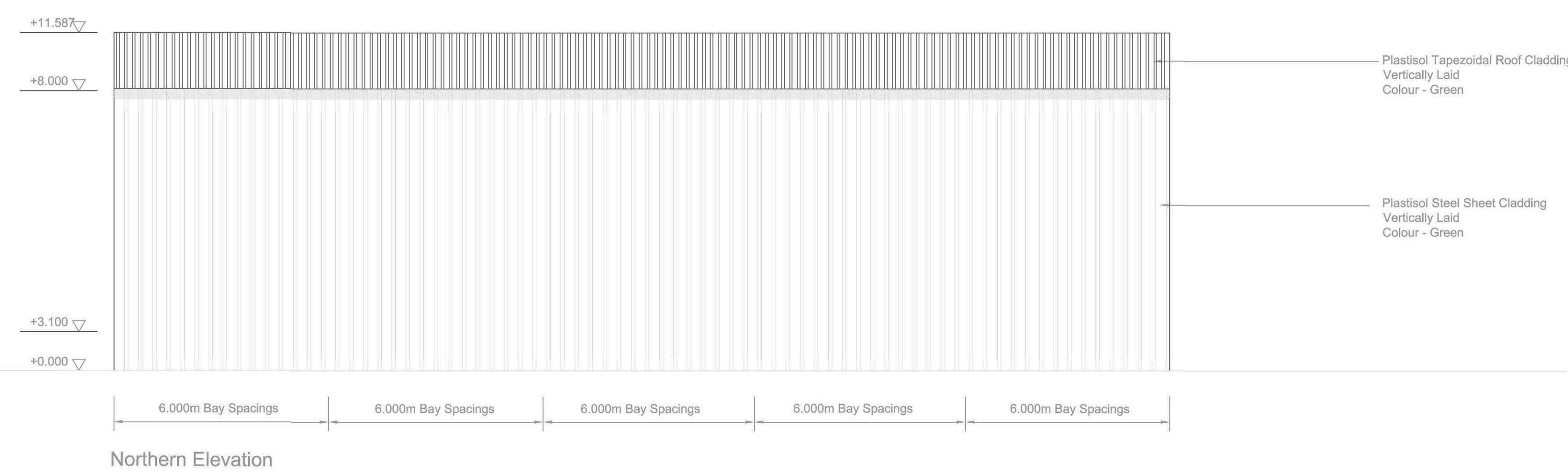
Northern Elevation
