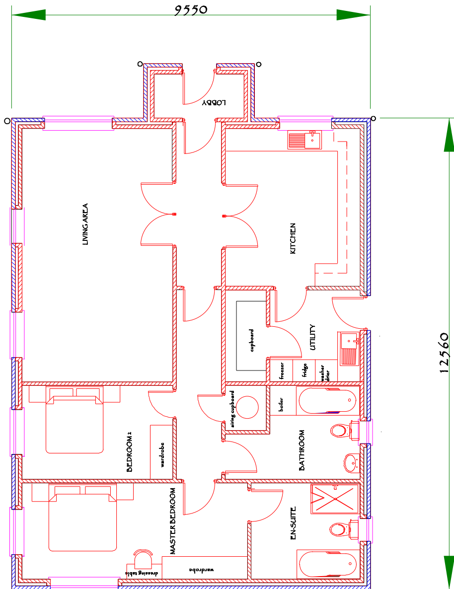
FLOOR PLAN
