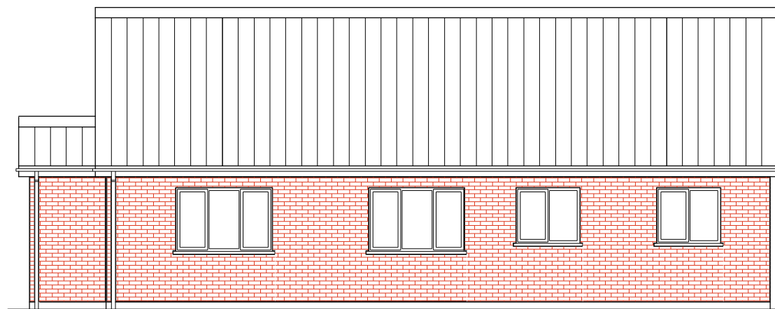
PROPOSED SOUTH WESTERN ELEVATION
