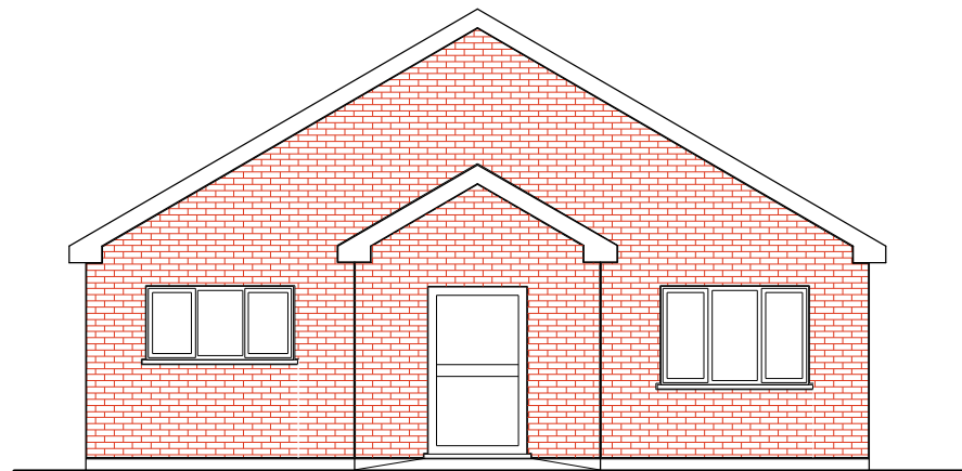
PROPOSED NORTH WESTERN ELEVATION
