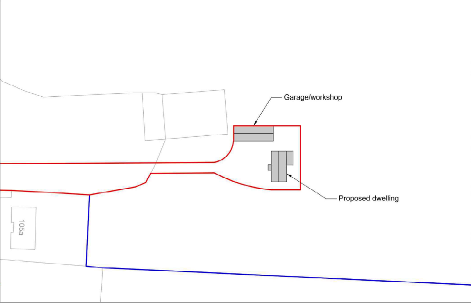
Proposed block plan - 1:500@A1
