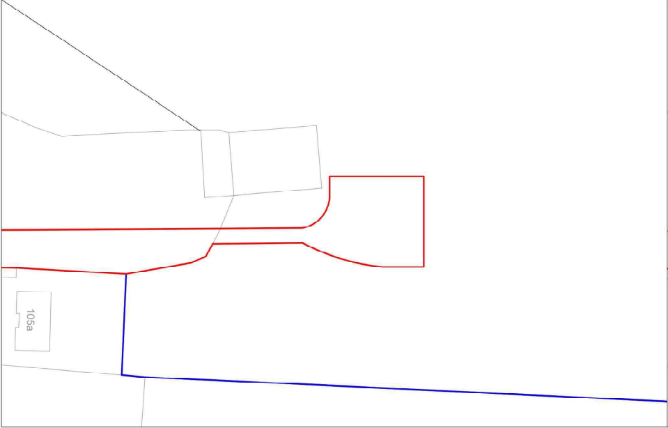
Existing block plan - 1:500@A1
