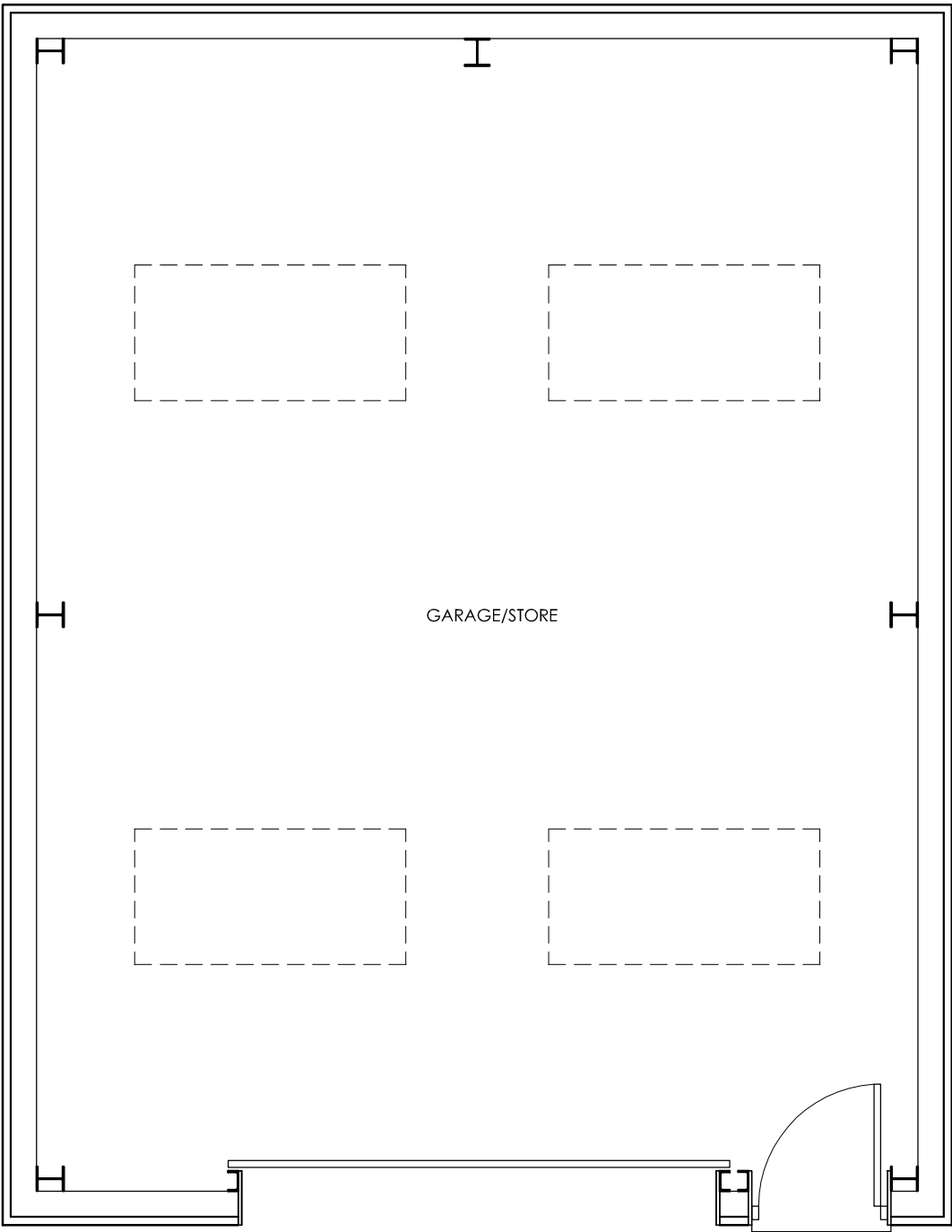
FLOOR PLAN 1:50
