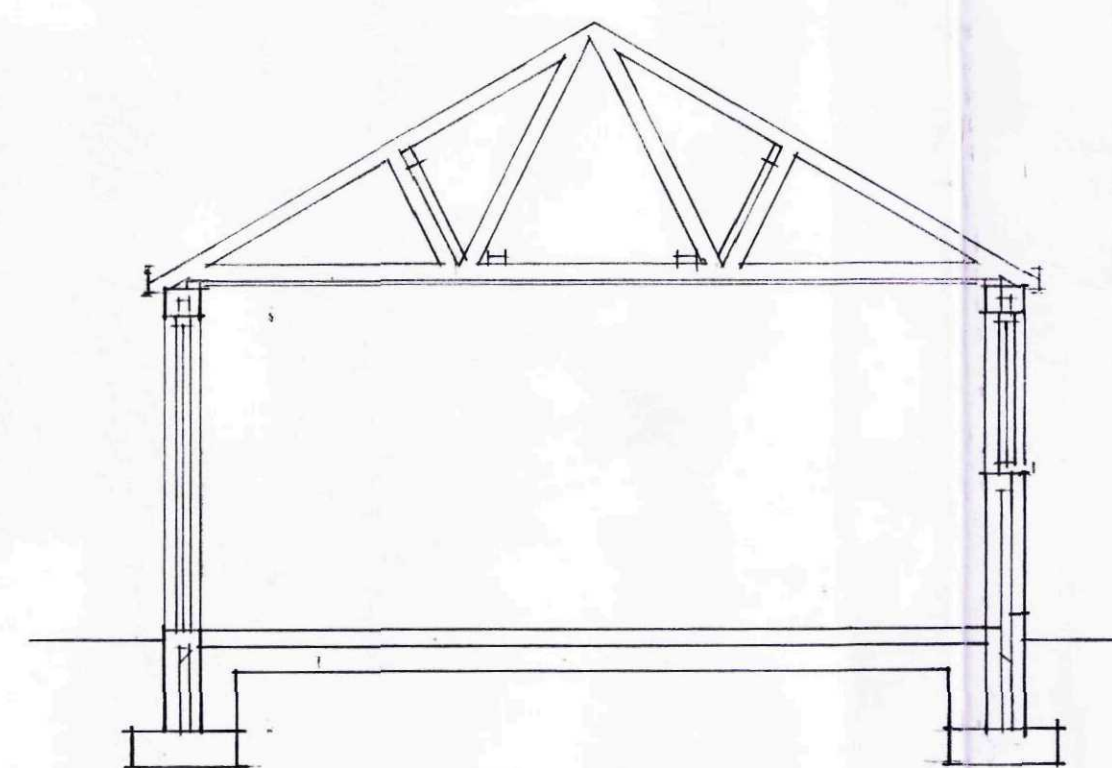
SECTION THRO GARAGE
