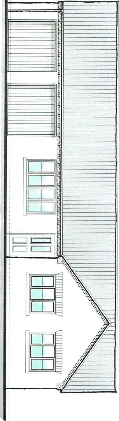
front elevation
