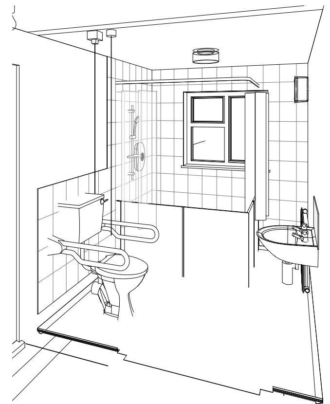
2 Shower Perspective
