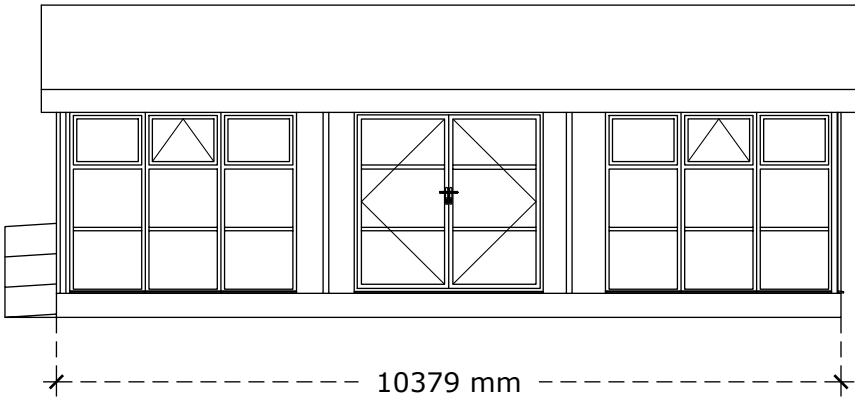
Front (E) elevation
