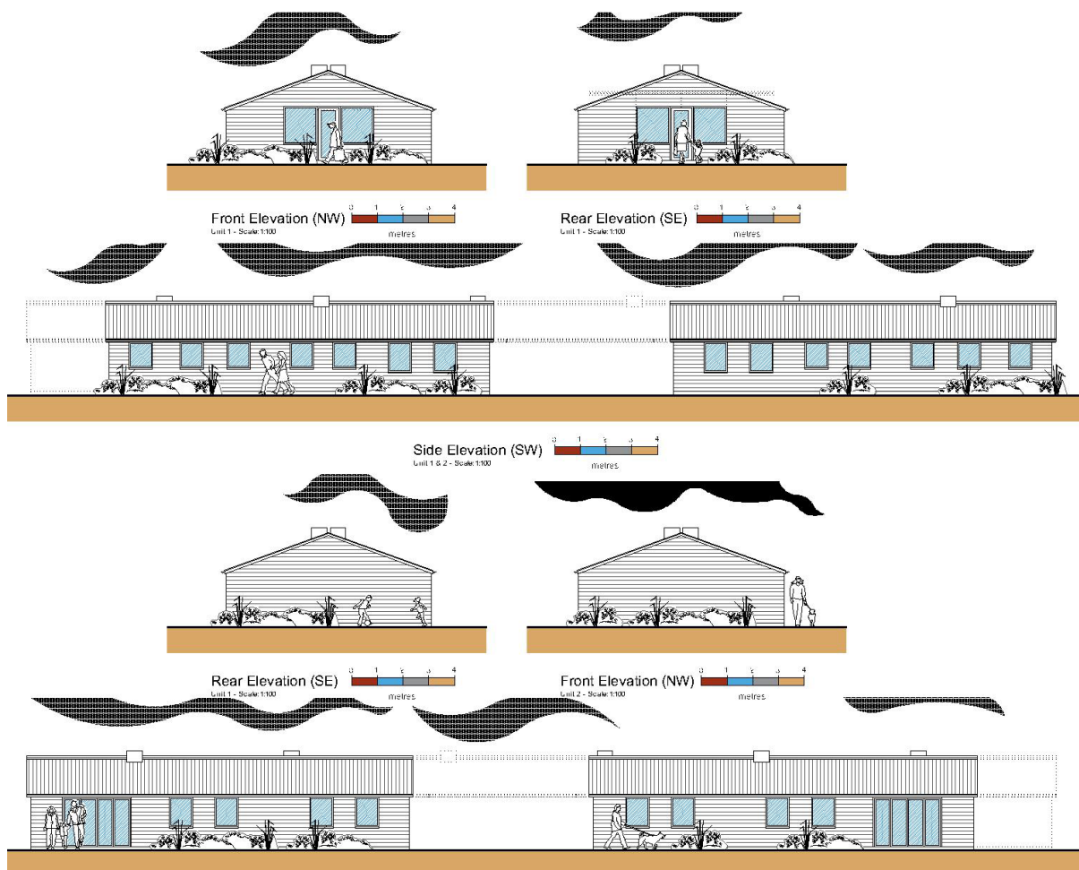
Figure 5 – Units 1-2 Proposed Elevations
