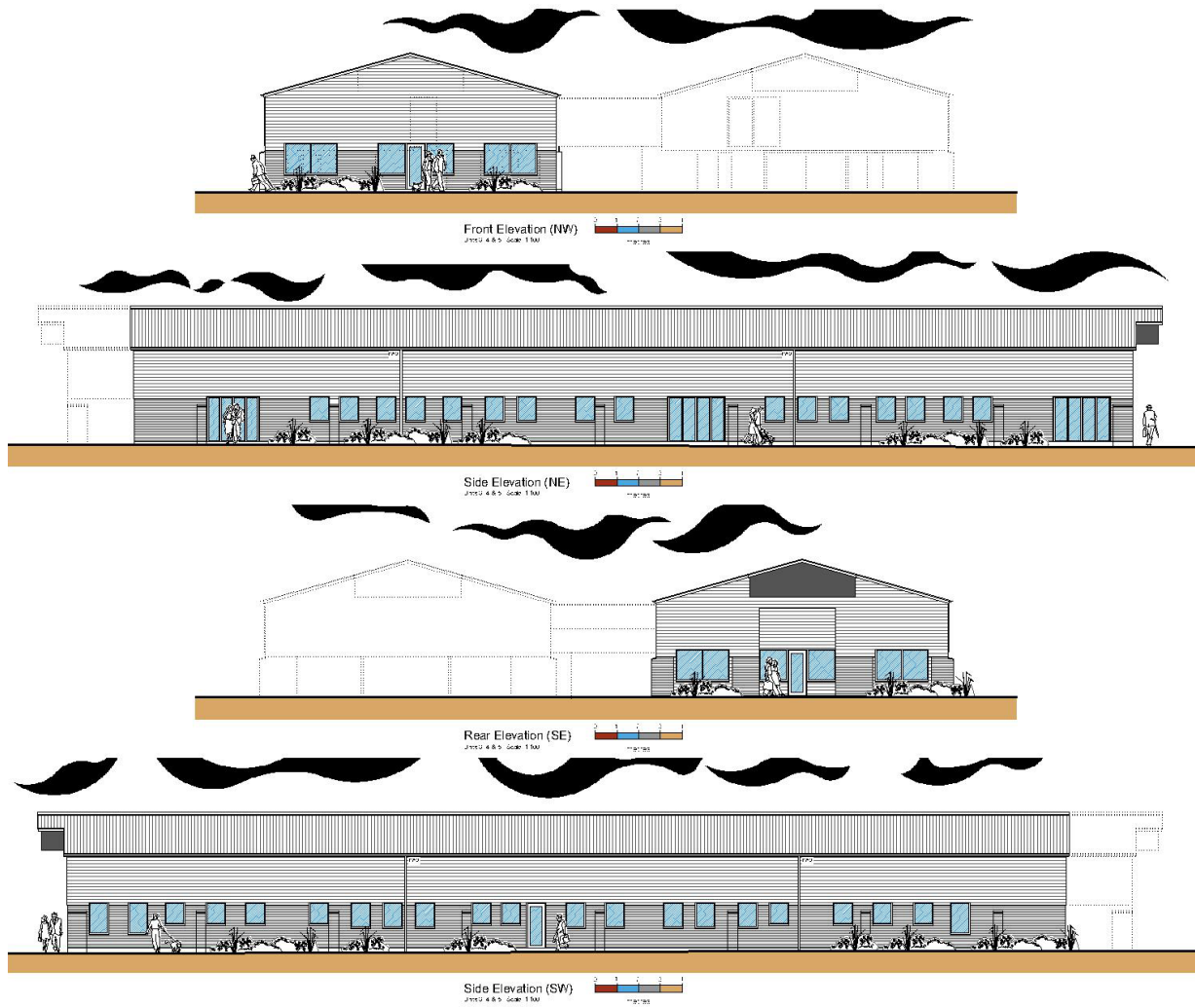
Figure 6 – Units 3-5 Proposed Elevations
