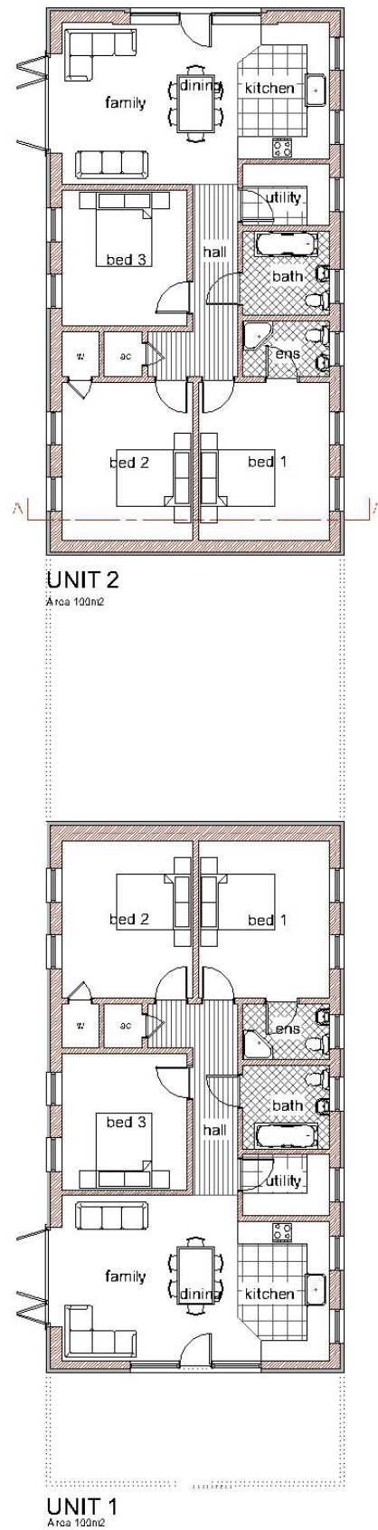
Figure 3 – Units 1-2 Proposed Floor Plan
