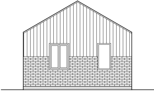
Back Elevation 1:100
