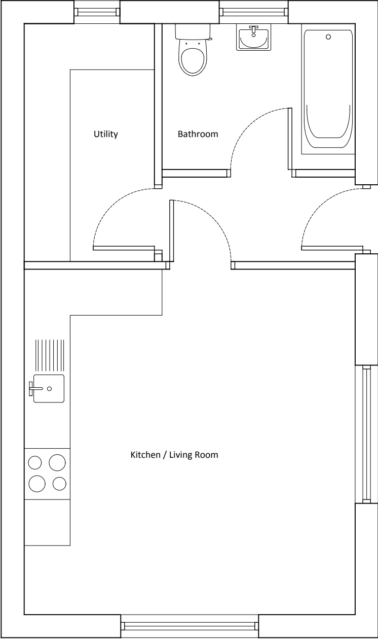
Floor Plan 1:50
