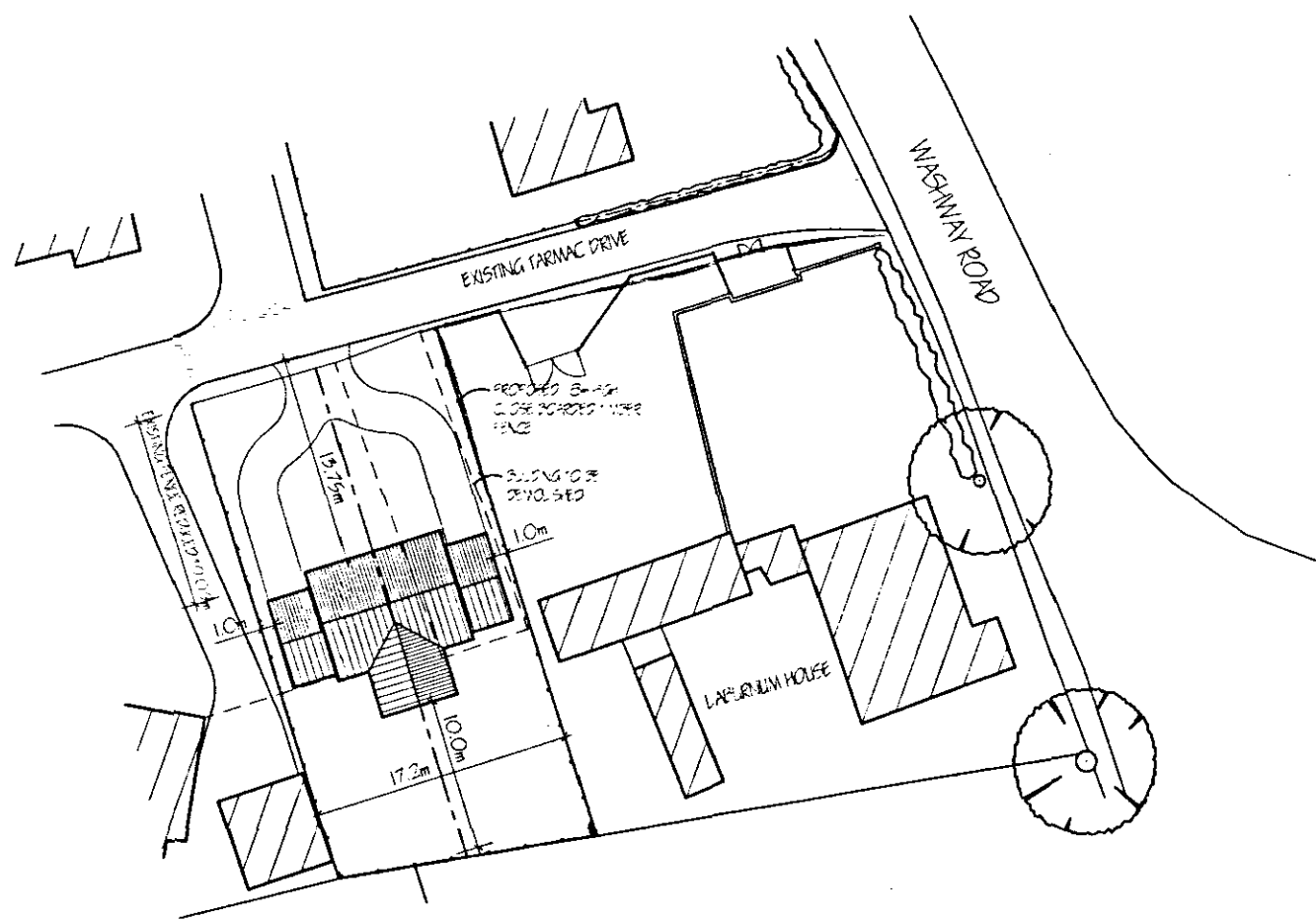
BLOCK PLAN 1:500 OPTION 1 PAIR OF SEMI-DETACHED HOUSES
