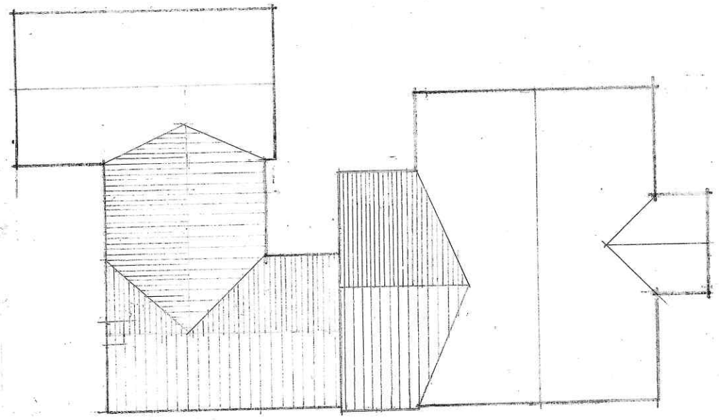
EXISTING ROOF PLAN 1:200
