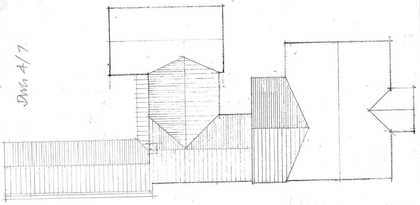
PROPOSED ROOF PLAN 1:200
