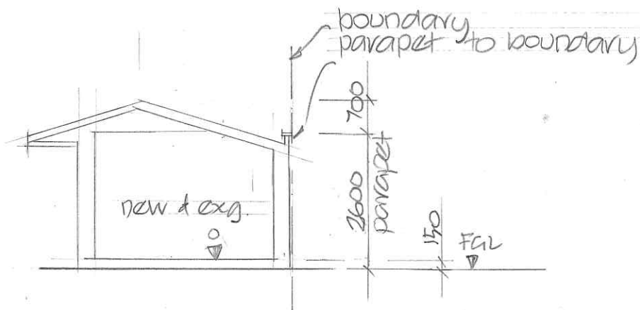
TYPICAL SECTION
